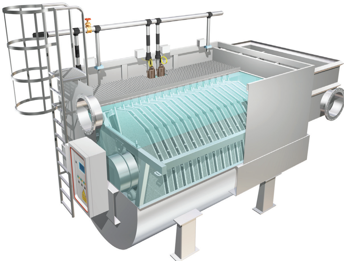
Evergreen cloth filter MSF16/80 in stainless steel tank
