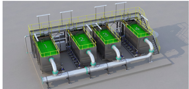
Crewe STW Evergreen cloth filters 3D render with inlet manifold and ground level control panels - Courtesy of Evergreen Water Solutions Design Team
